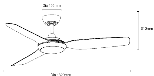
13220mm (52") Model
